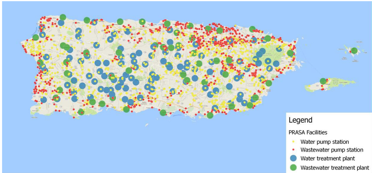
Figure 68. PRASA System Damage by Hurricanes Irma and María 175
