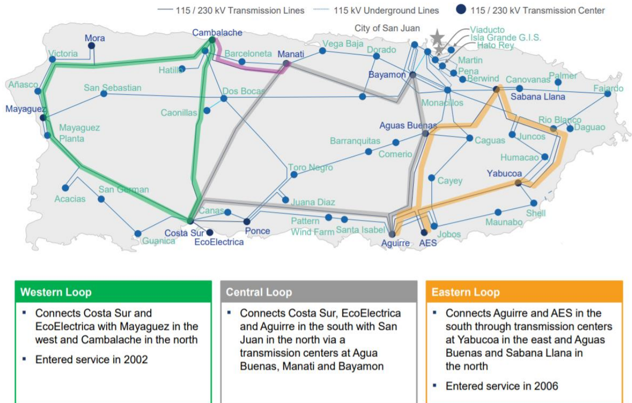
Figure 58. Map of PREPA transmission and distribution lines. Source: 2019 Fiscal Plan for the PREPA
